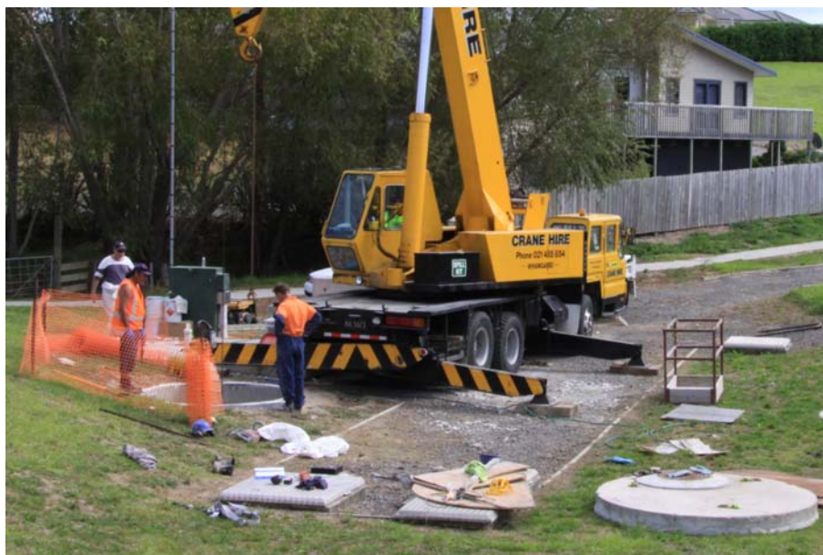
Photograph 9: Top off manhole, and preparing to install fiberglass liner.
